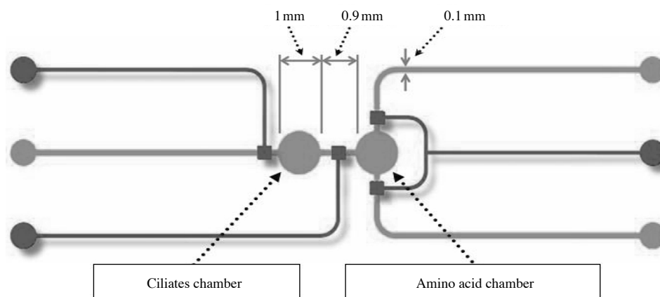
Figure 1. The microfluidic system used as a ciliate sensor. The lower layer represents the fluidic channel, while the upper layer is the pneumatic layer that controls the valves (the squares).
