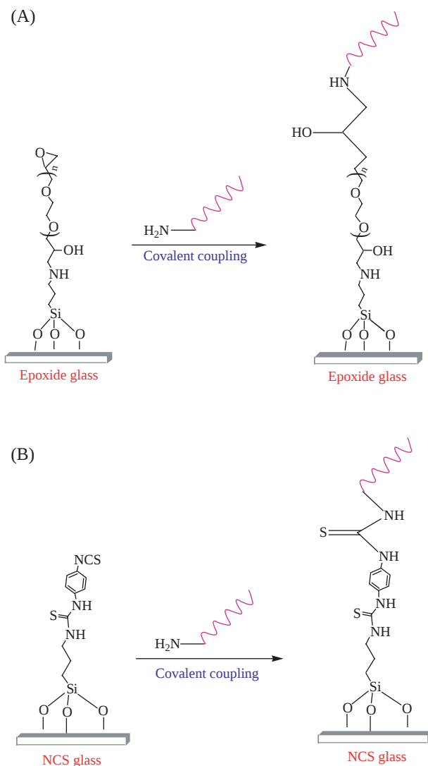
Figure 2. Immobilization strategy of capture DNA on (A) epoxide- and (B) NCS-activated glasses.
