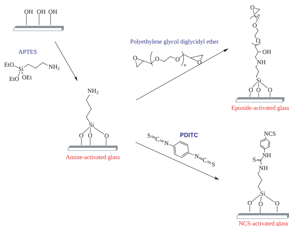
Figure 1. Preparation of epoxide- and isothiocyanate (NCS)-activated glasses.
