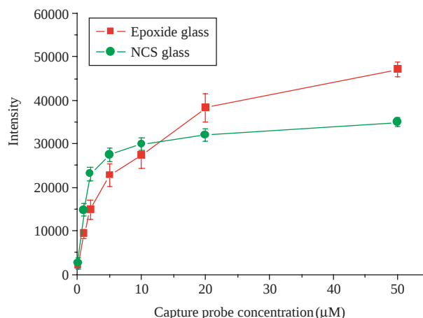
Figure 3. Immobilization capacities of epoxide- and NCS-activated glasses.
