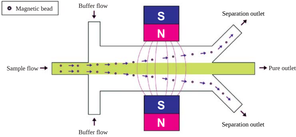
Figure 1. A schematic diagram of the dipole magnet sorter used in the experiment.
