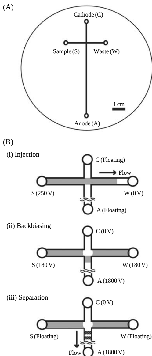
Figure 3. (A) A capillary electrophoresis microchip to separate PCR products by cross injection process. This 10 cm dia. microdevice consists of a glass-glass layer and is etched to form a cross fluidic microchannel and four reservoirs (an anode, a cathode, a sample, and a waste). (B) CE operation on a microdevice. (i) sample injection step (ii) backbiasing step and (iii) separation step (▨: ET dye-labeled PCR product, ▨: Single dye-labeled PCR product).
