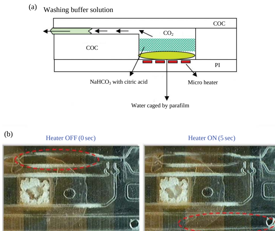
Figure 4. (a) Working principle of the COC-based micropump and (b) images showing the fluid movement by the fabricated micropump.
