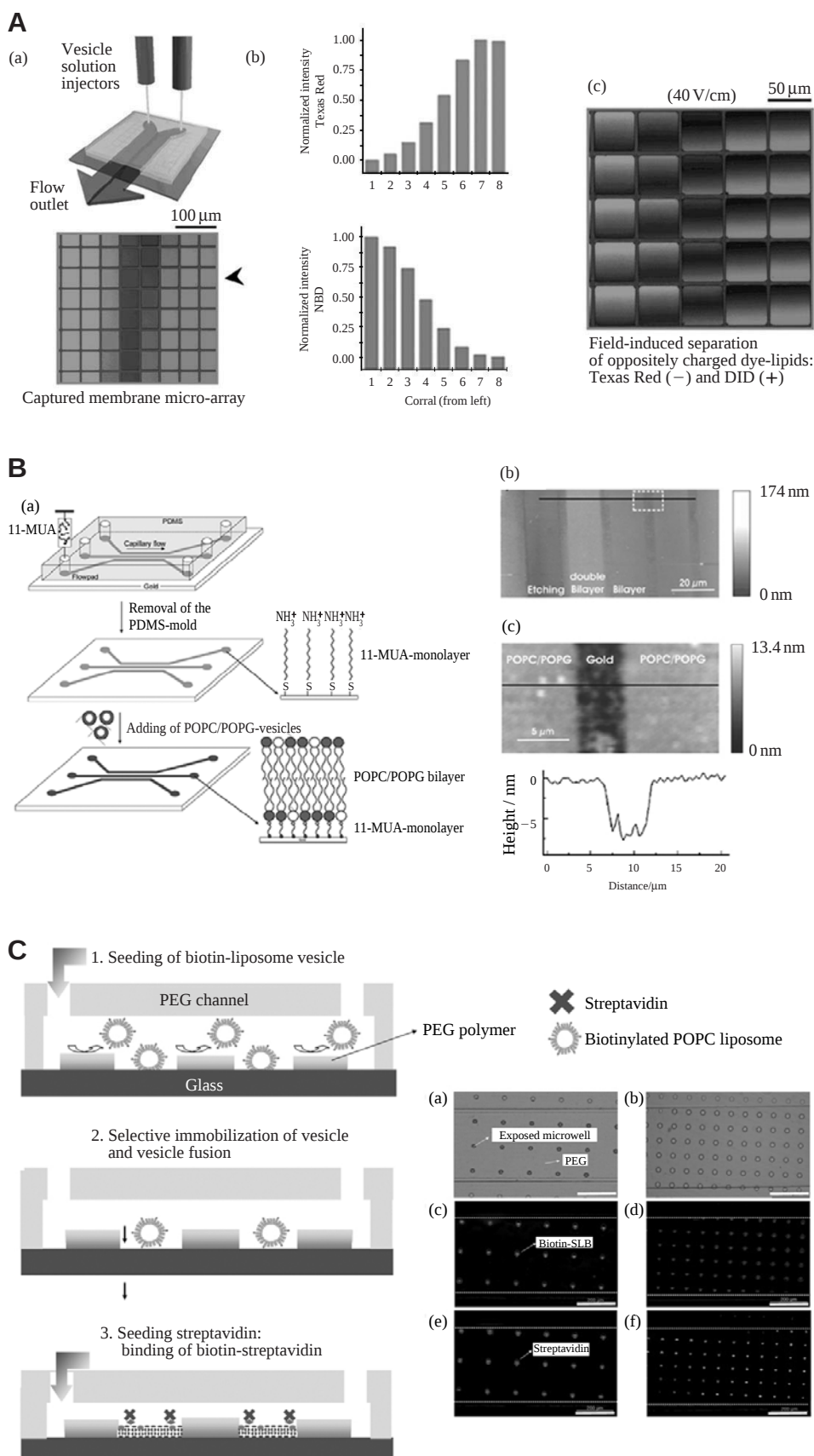
Figure 3. Microarrays of lipid membrane within a microfluidic channel. (A) Schematic illustration of the converging flow configuration used to produce the limited mixing of two types of vesicles in solution. Reprinted with permission from 67 . (B) Microstructuring of lipid bilayers on gold surfaces by MIMIC employing chemically modified PDMS. Reprinted with permission from 68 . (C) Supported bilayer membranes (SBMs) by using capillary molding of a PEGbased polymer within a PEG channel. Reprinted with permission from 31 .
