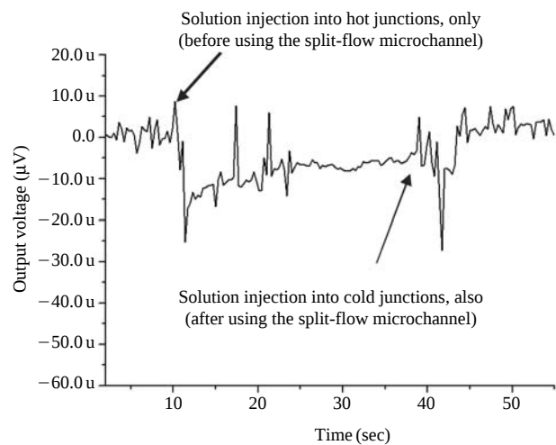
Figure 6. Performance of the split-flow microchannel. Thermal noises due to the solution injection itself are compensated by using the split-flow microchannel. This graph shows the recovery of output voltages to a zero level through the split-flow microchannel.
