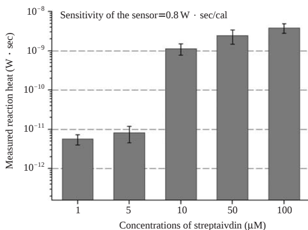
Figure 10. The measured output signals according to the concentration of streptavidin; the sensitivity of the sensor was 0.8 W · sec/cal.
