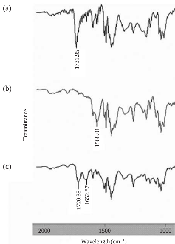
Figure 1. The FT-IR spectra of (a) resin 3 before saponification, (b) resin 3 after saponification, and (c) resin 4.
